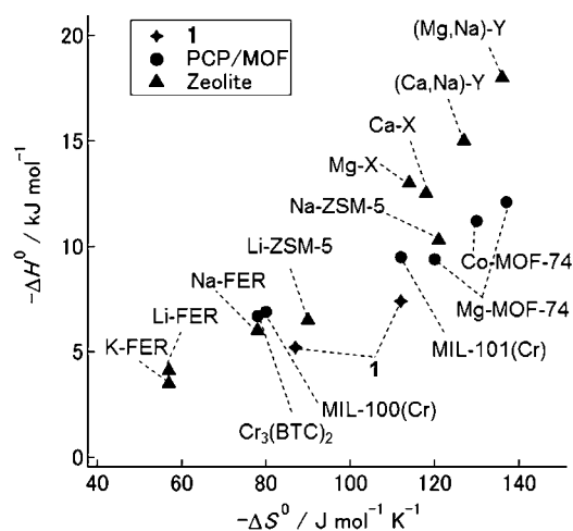
Figure 5. Standard adsorption enthalpy versus entropy for hydrogen adsorption on 1 , PCPs/MOFs reported previously, and zeolite. The points are taken from Table S4 in the Supporting Information.
